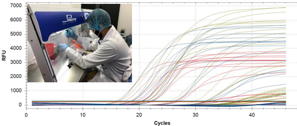
Amplification
